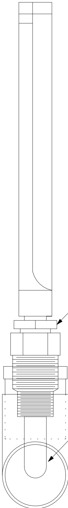
SIDE VIEW OF STN-100 IMMERSION THERMOMETER
